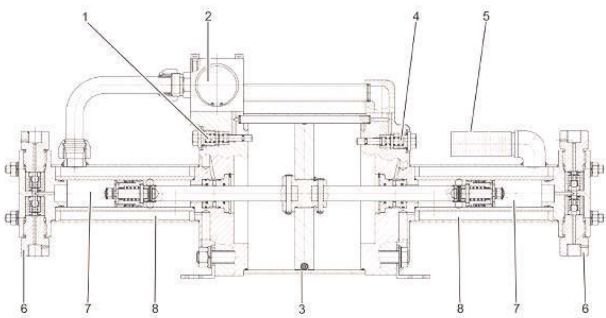
Fig. Maximator booster, type DLE 15
