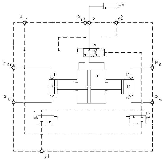
Fig. Connection diagram for double-acting booster
