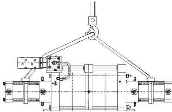
Fig. 8 DLE lifting points
