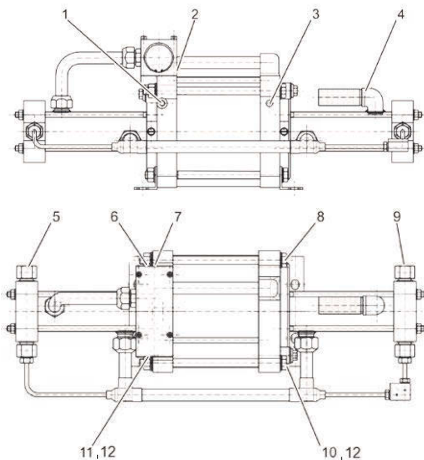
Fig. Ports for combined booster
