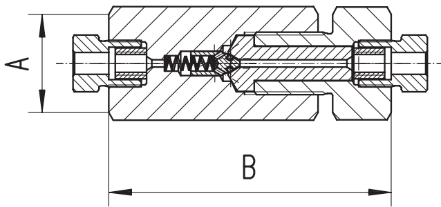
O-Ring Check Valves
