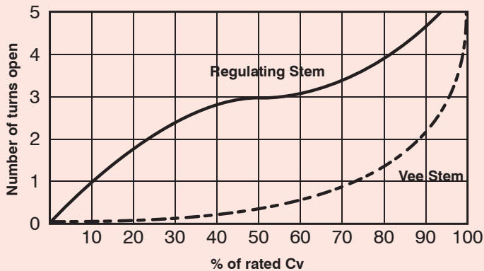
Flow Coefficient Reference Curves (Cv)
