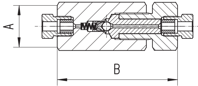
Ball Check Valves
